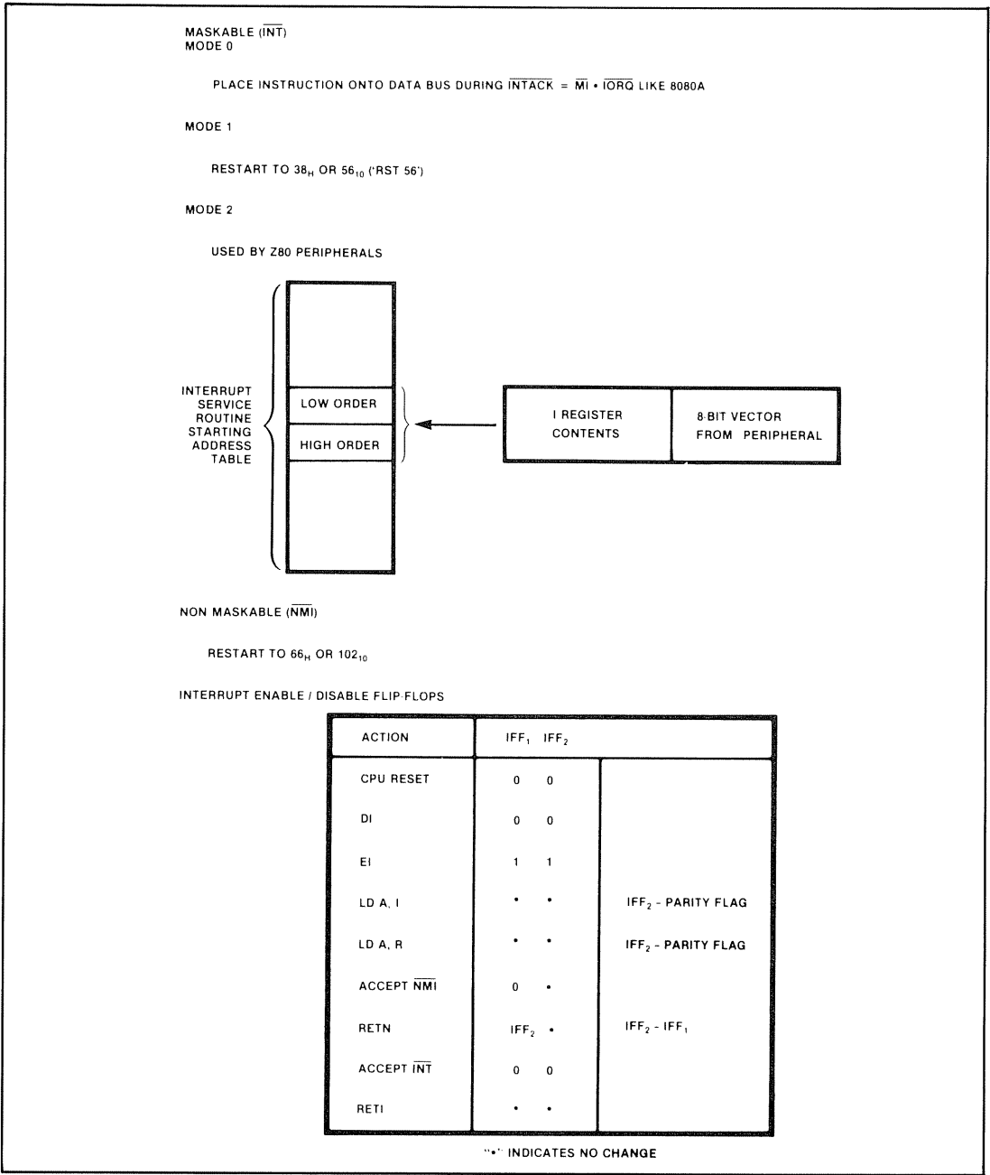
Figure A-3. Z80 interrupt structure
